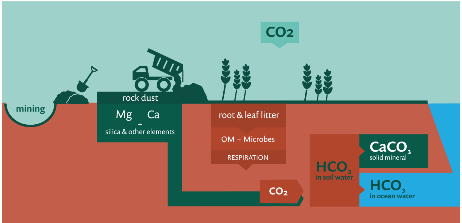
Figure 1. The ERW Process
